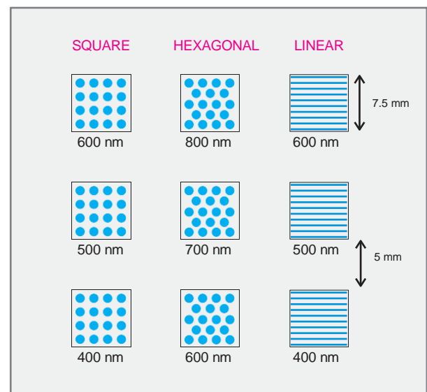
(Layout of MHSL400-800 showing pattern periods. Drawing not to scale)
